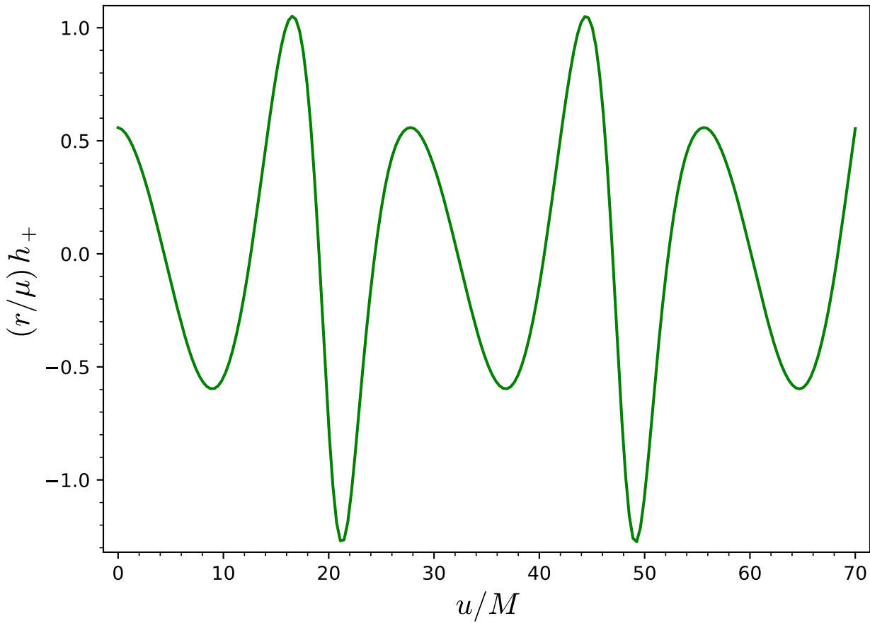
GW from ISCO, a = 0.9M
