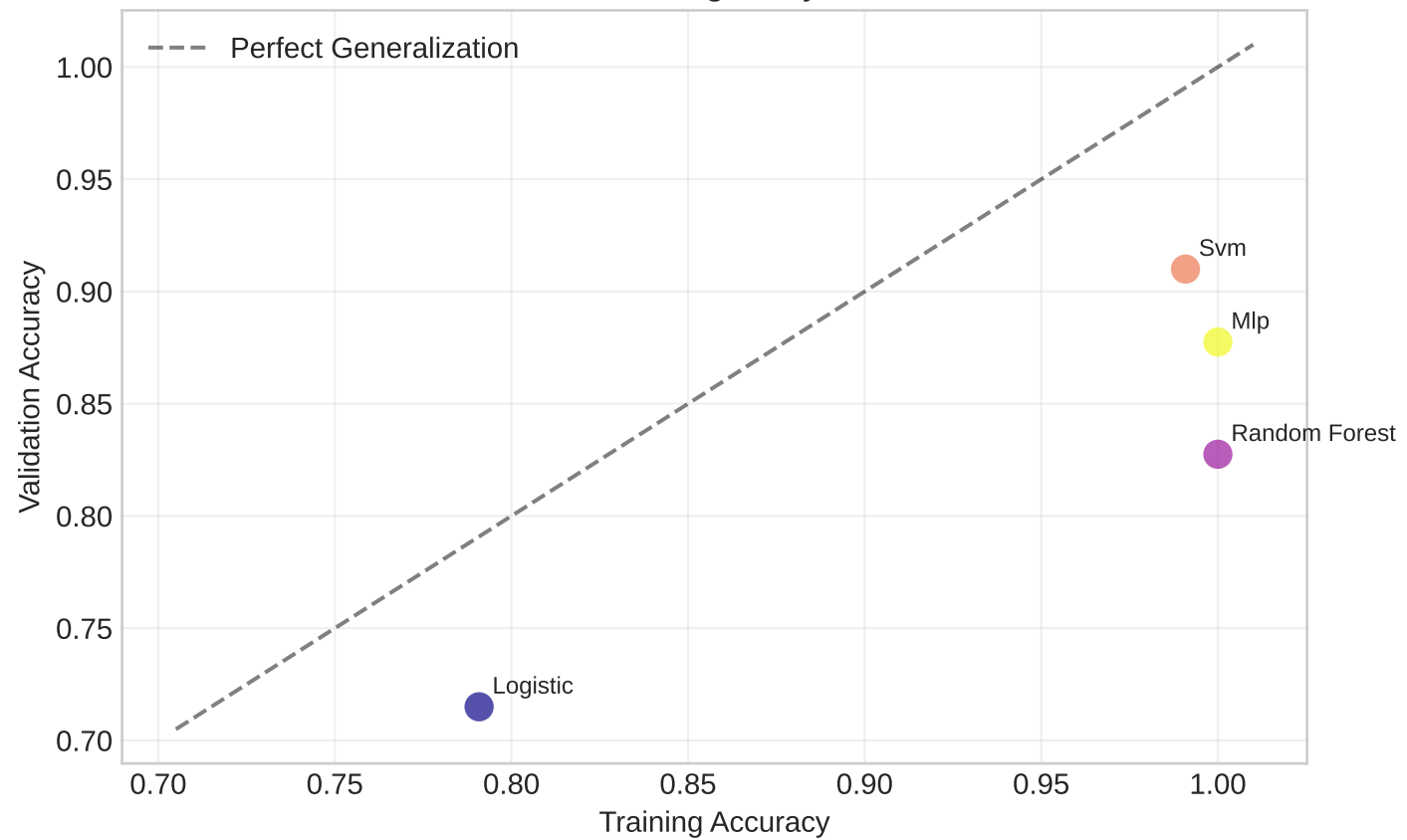
Overfitting Analysis
