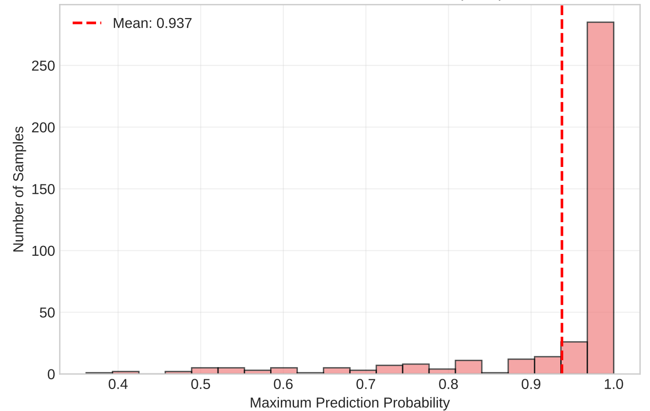
Overfitting Analysis
