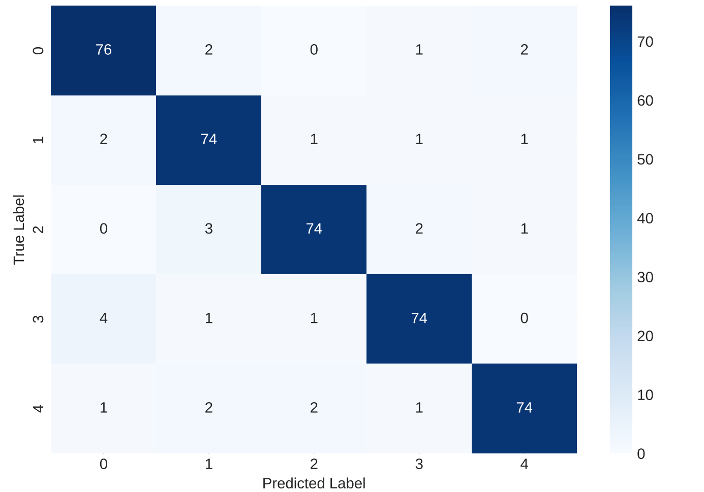
Confusion Matrix - Svm
