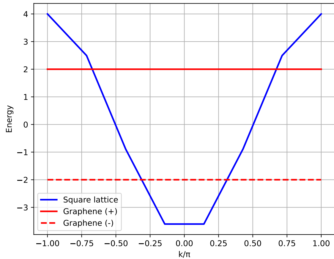
Electronic Band Structure
