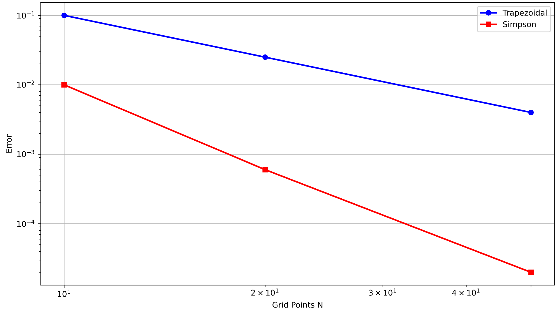
Numerical Integration Convergence
