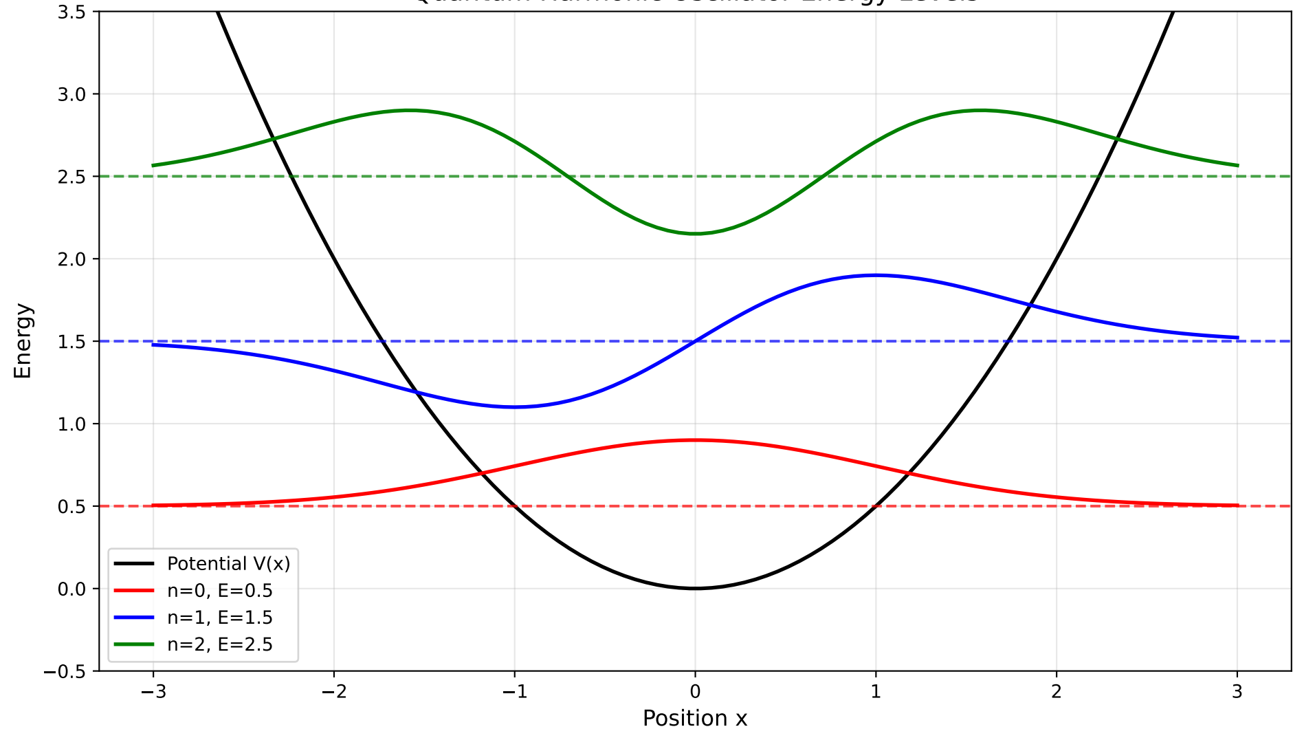
Quantum Harmonic Oscillator Energy Levels
