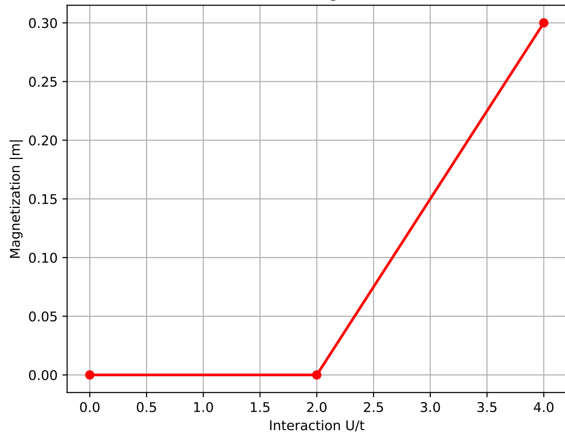
Hubbard Model: Magnetic Transition
