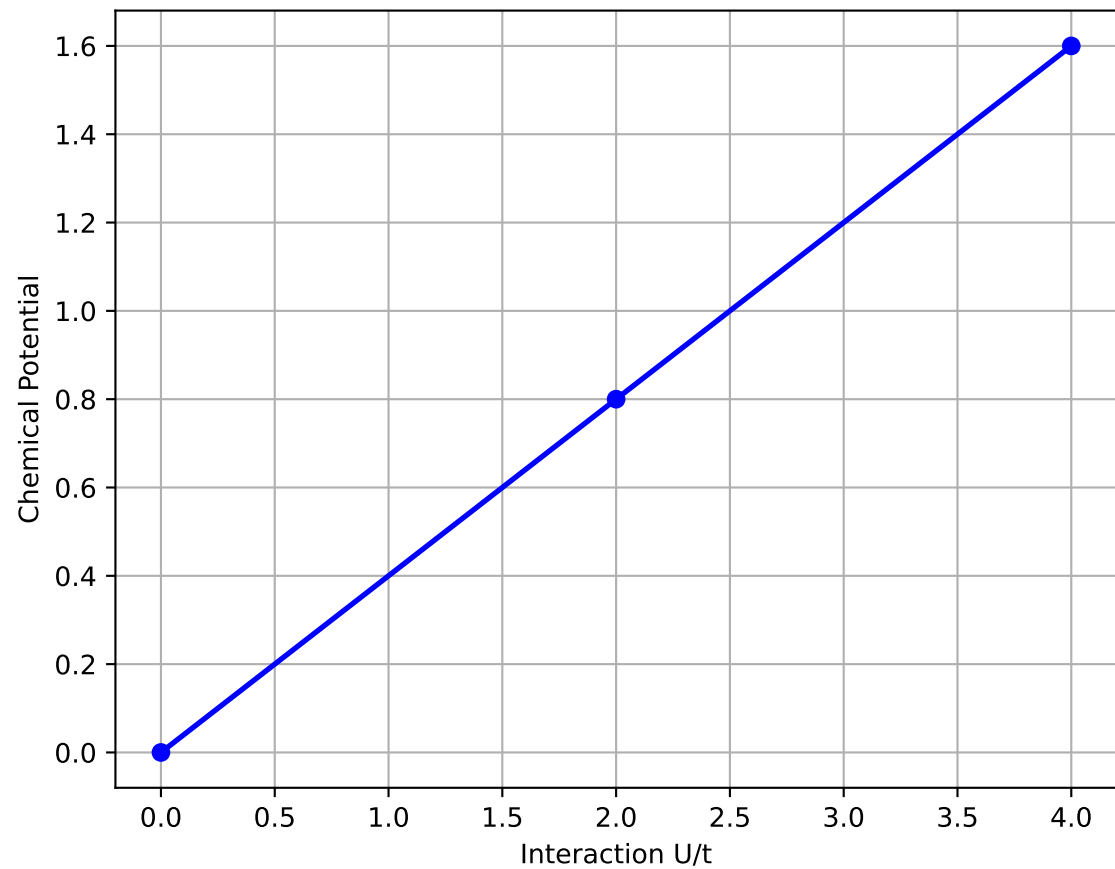
Chemical Potential vs Interaction
