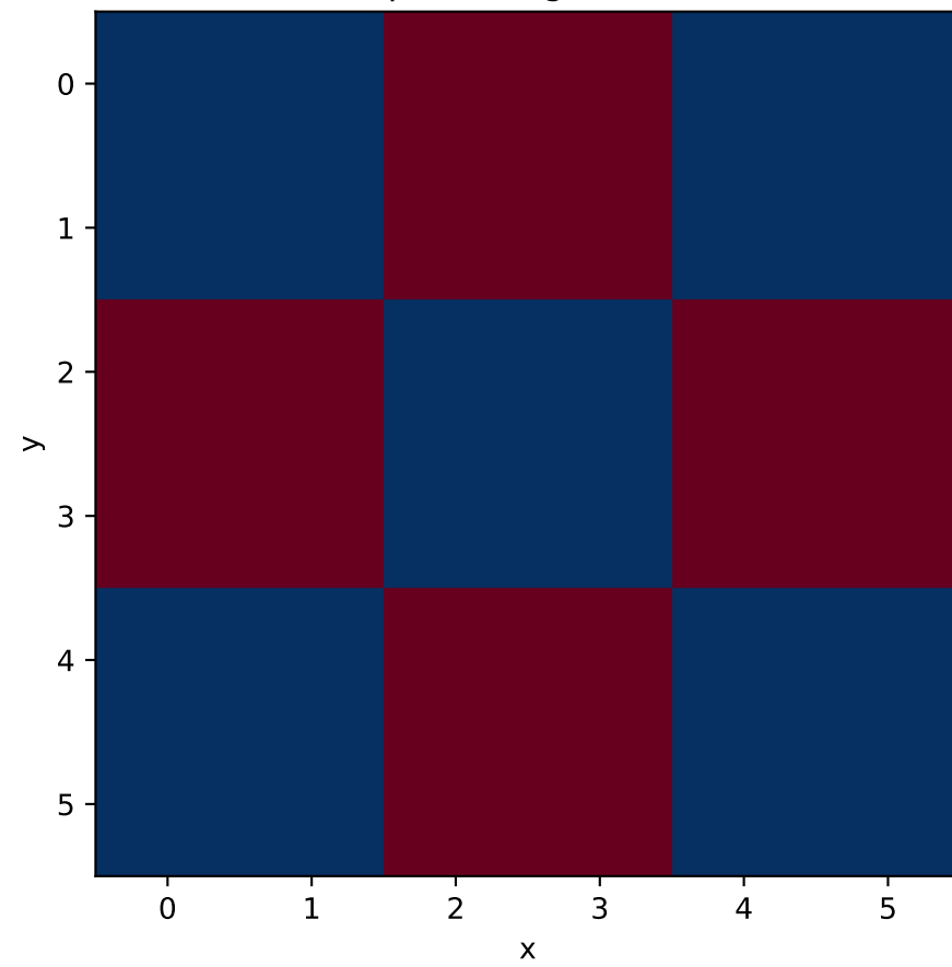
Spin Configuration
