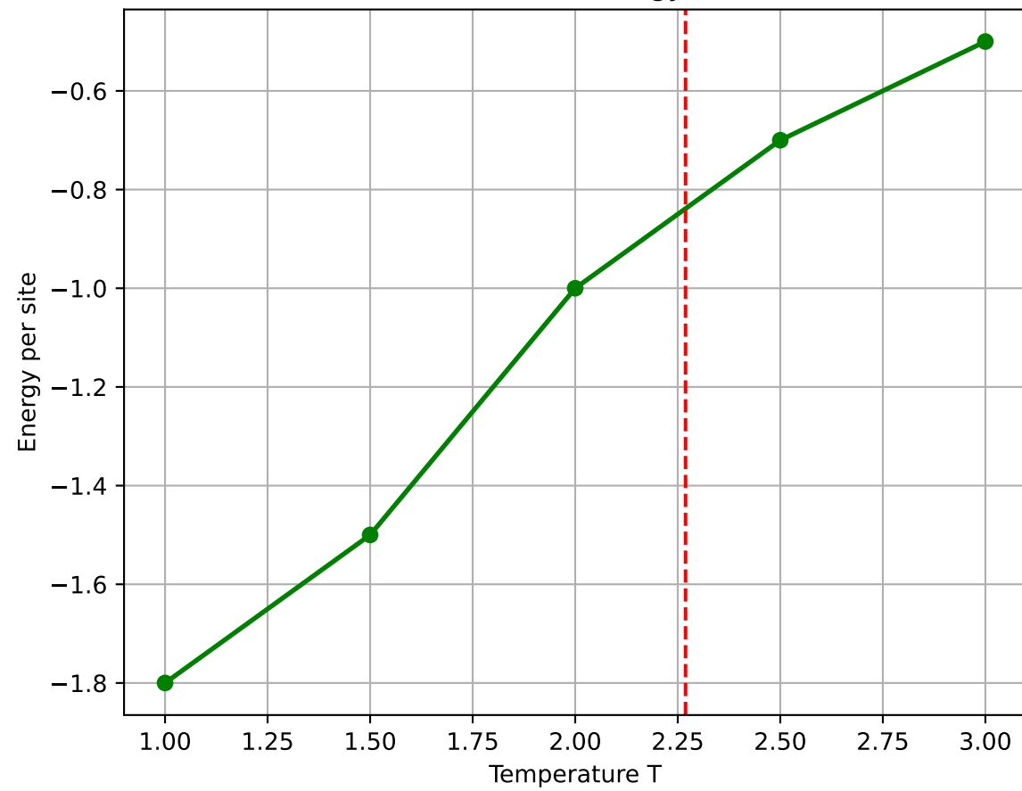
Internal Energy
