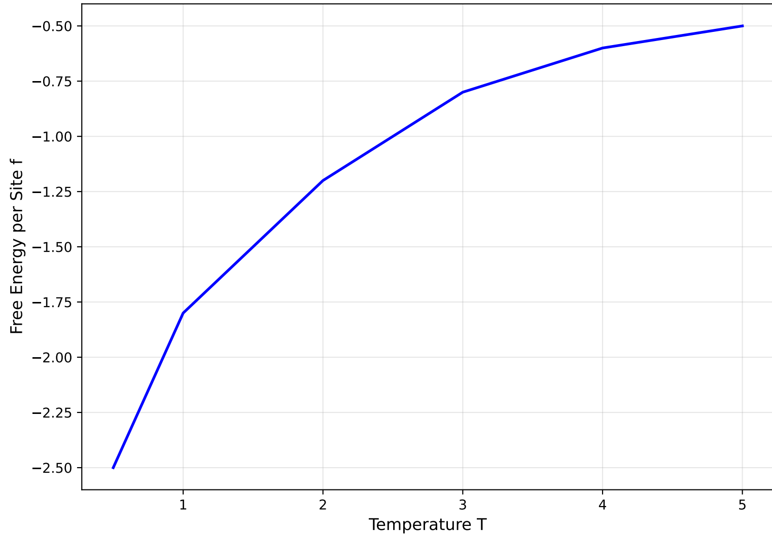
1D Ising Model: Free Energy (Exact Solution)
