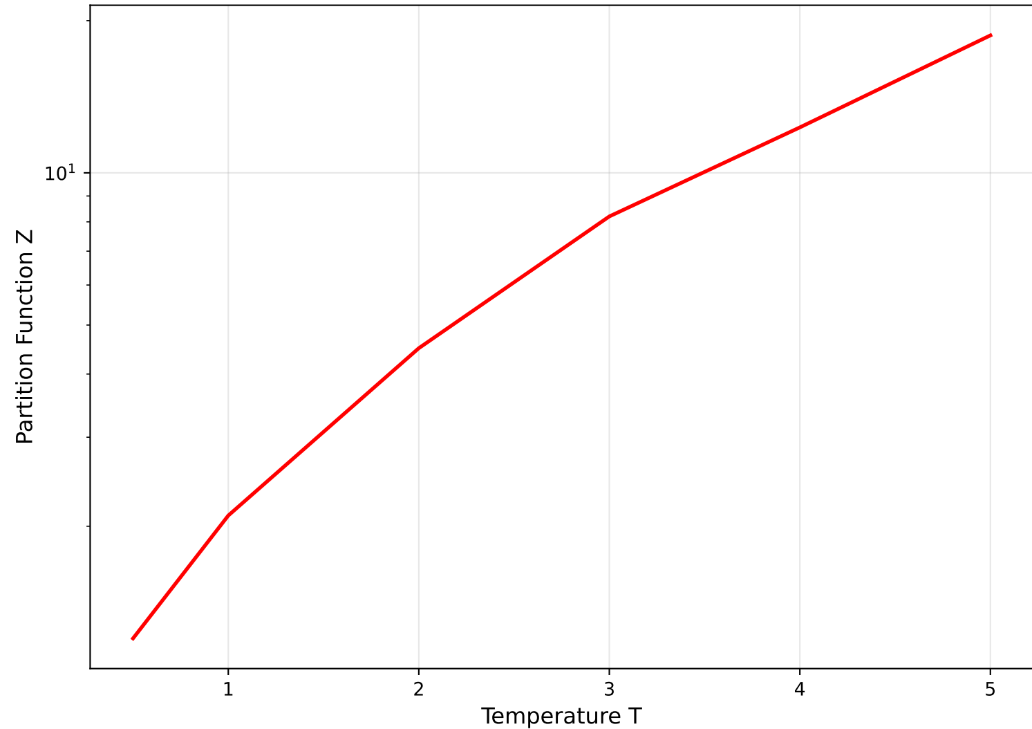
Partition Function: Statistical Weight
