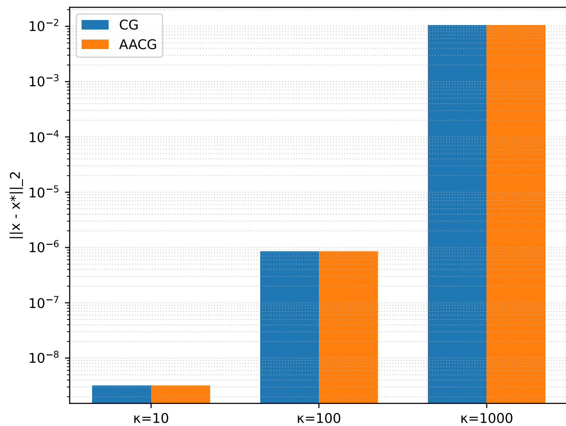
Final solution error
