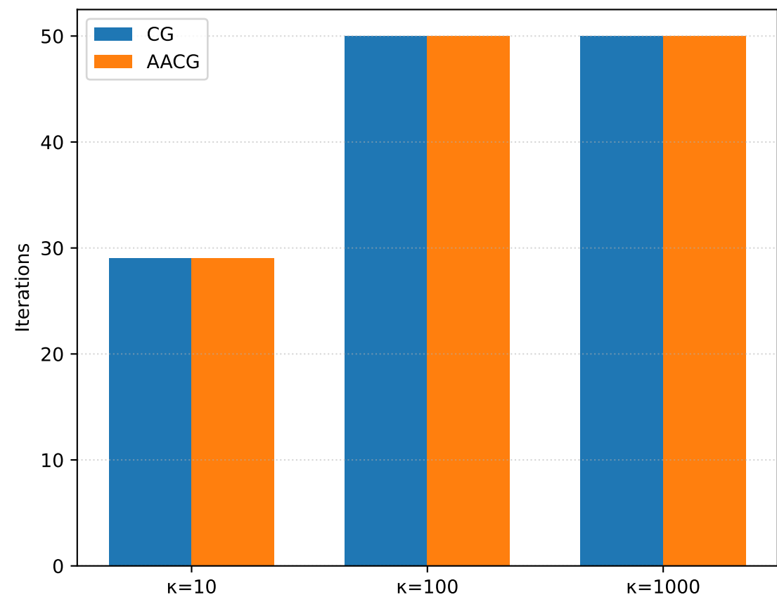
Iteration counts to tolerance
