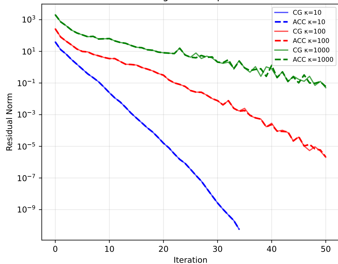
Convergence Comparison
