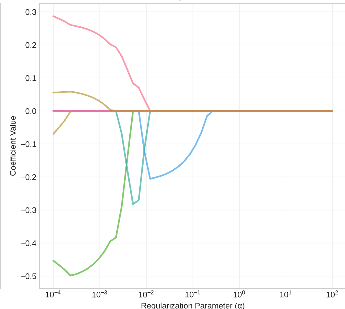
Lasso Regularization Path
