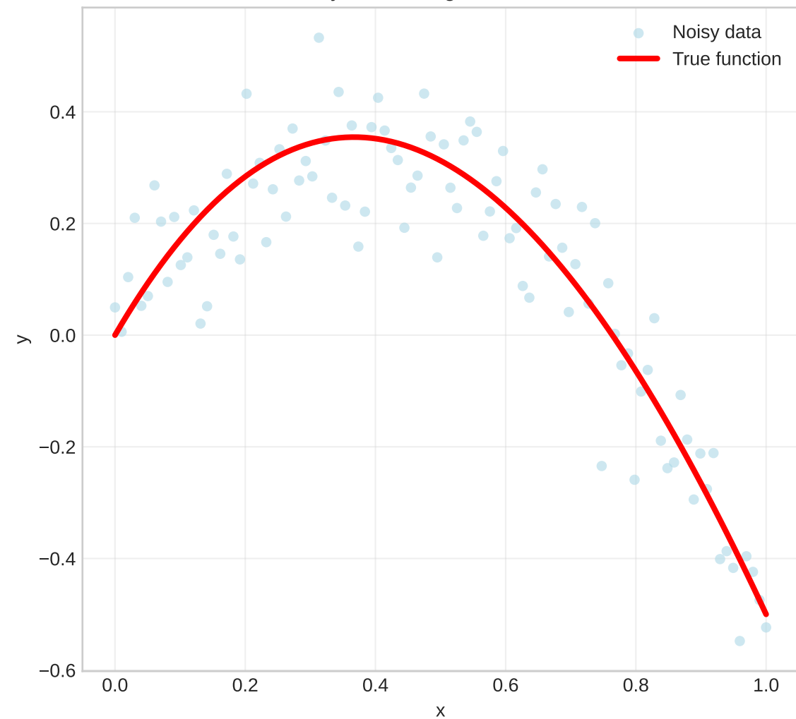
Polynomial Regression Data
