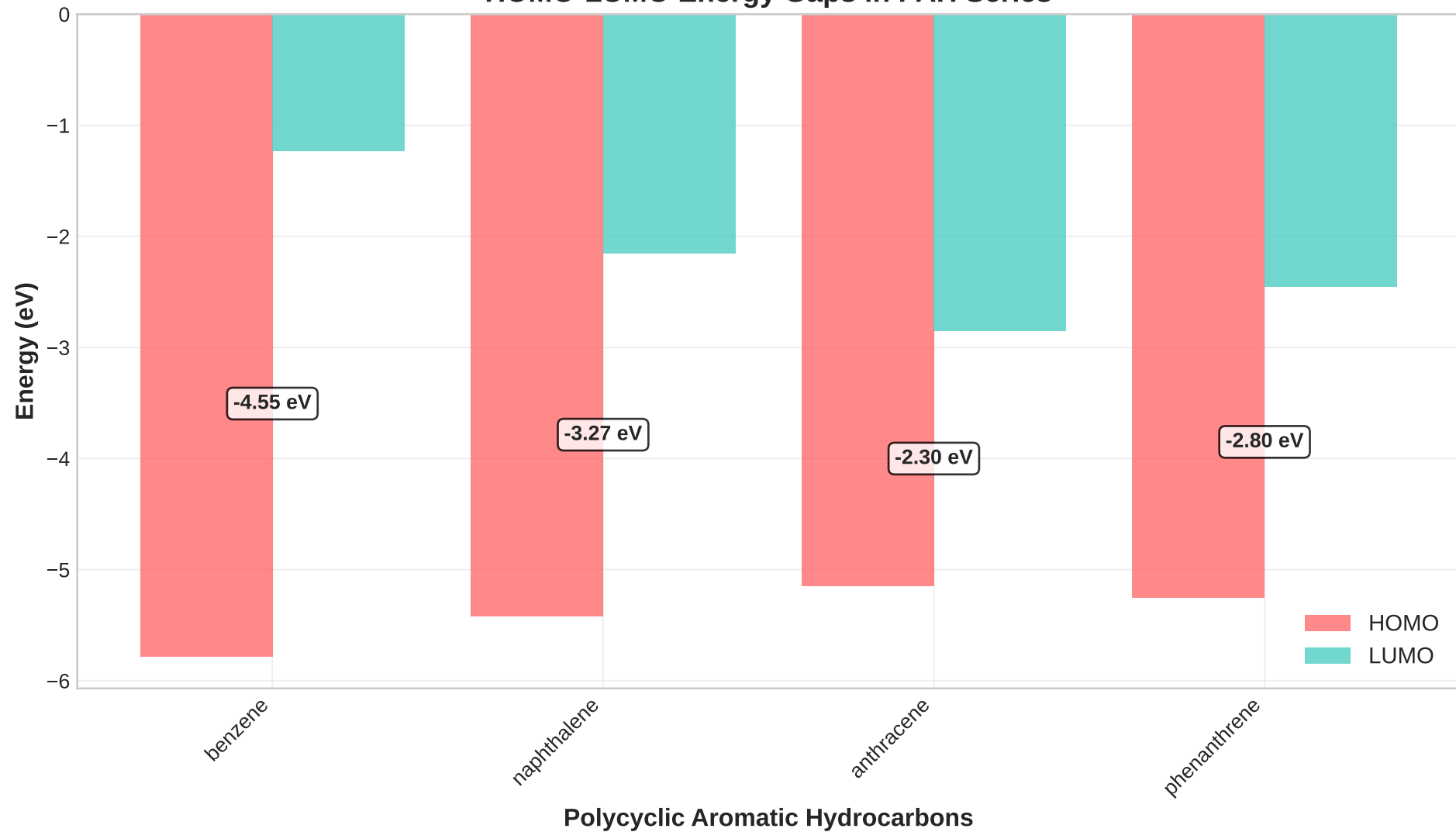
HOMO-LUMO Energy Gaps in PAH Series
