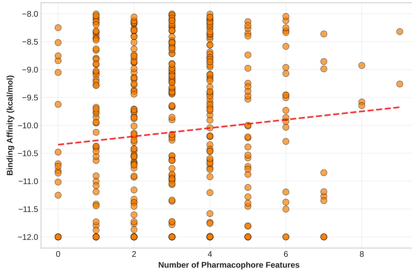
Structure-Activity Relationship
