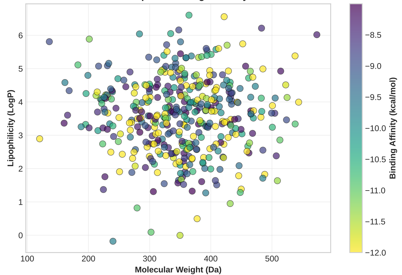
Structure-Activity Relationship
