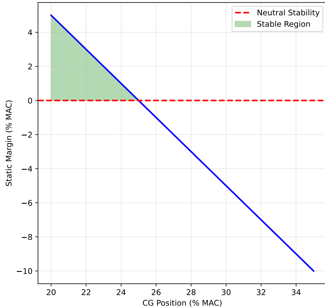
Longitudinal Static Stability
