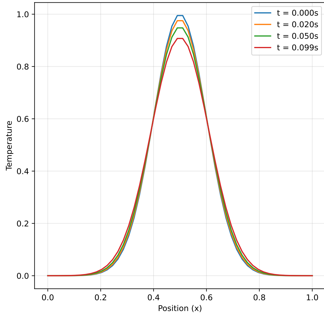
1D Heat Equation Solution
