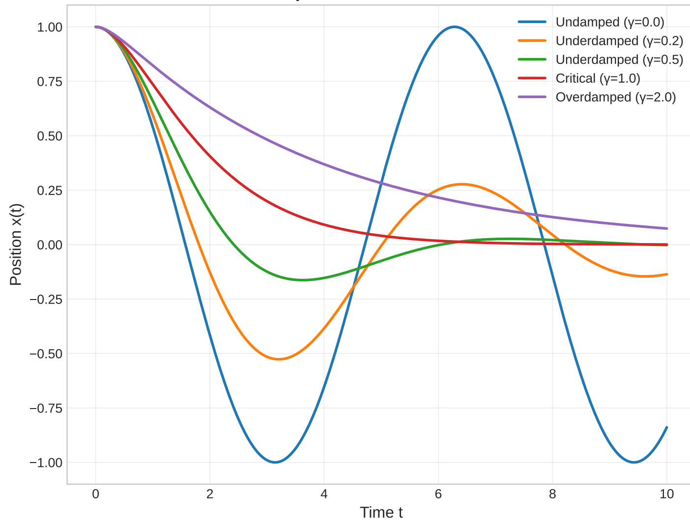
Damped Harmonic Oscillator
