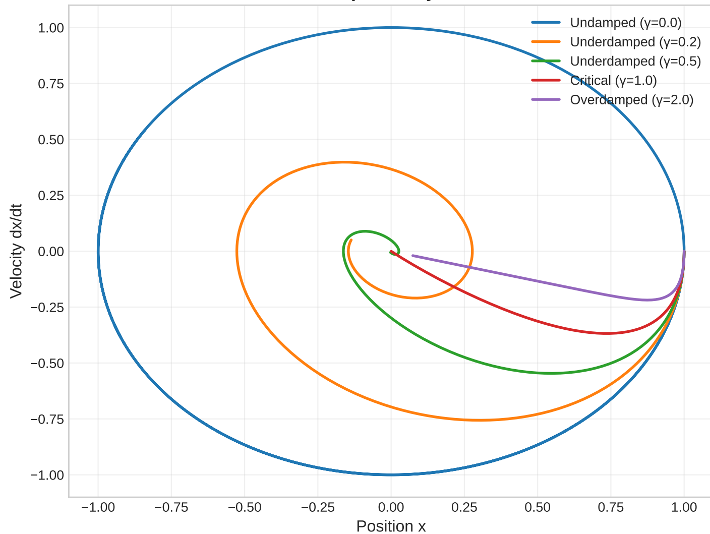
Phase Space Trajectories
