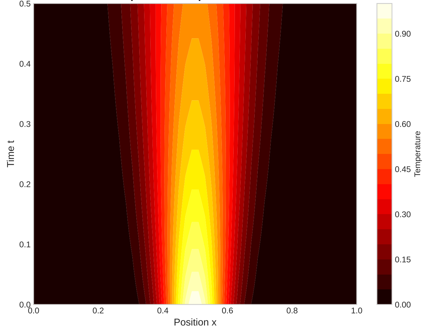
Heat Equation: Temperature Evolution
