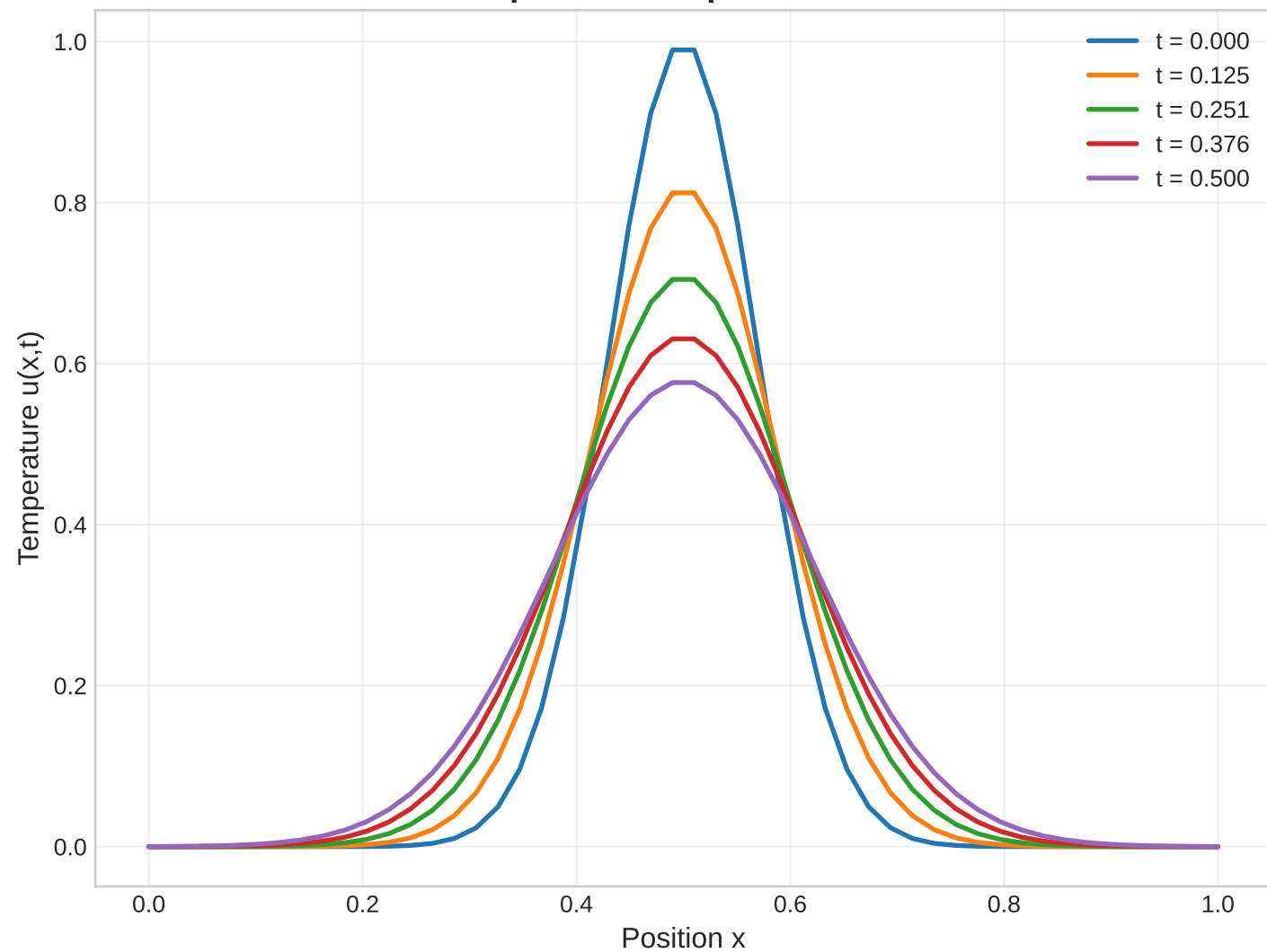
Heat Equation: Temperature Profiles
