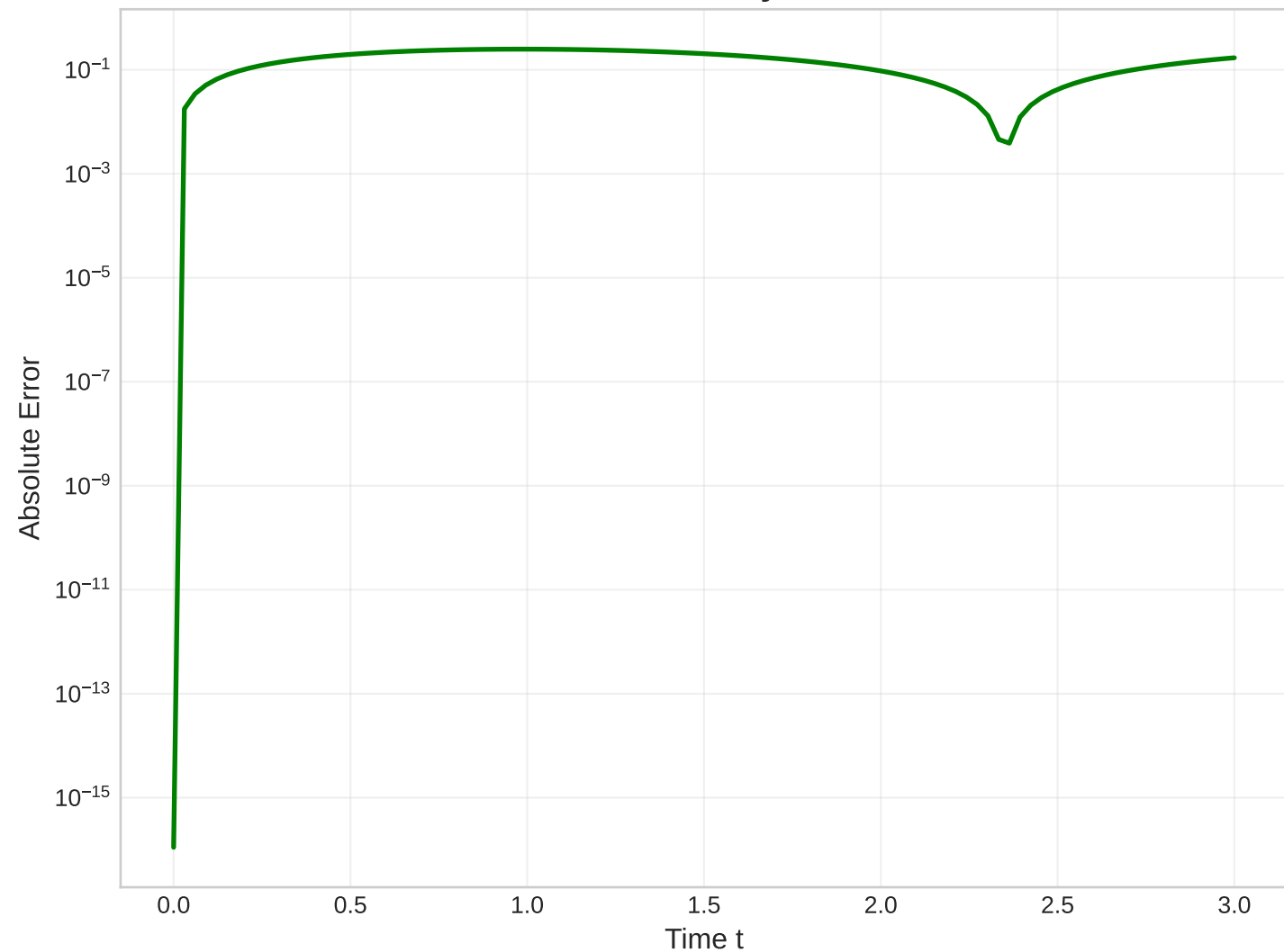
Numerical vs Analytical Error
