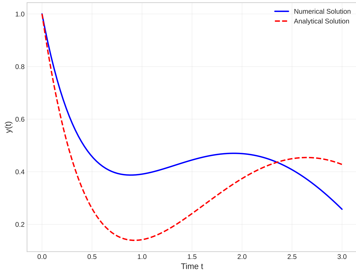
First-Order Linear ODE Solution
