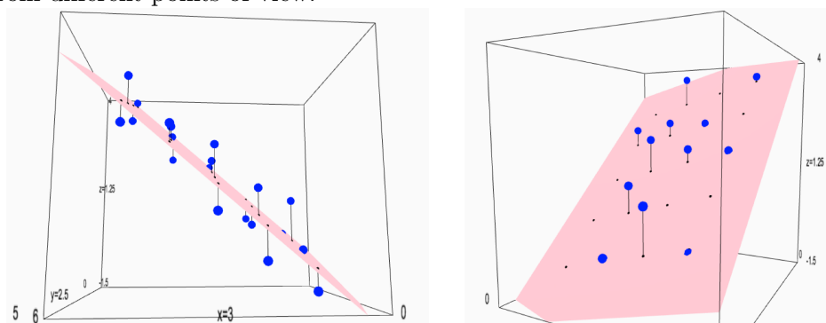
Two Views of the Best-Fit Plane
